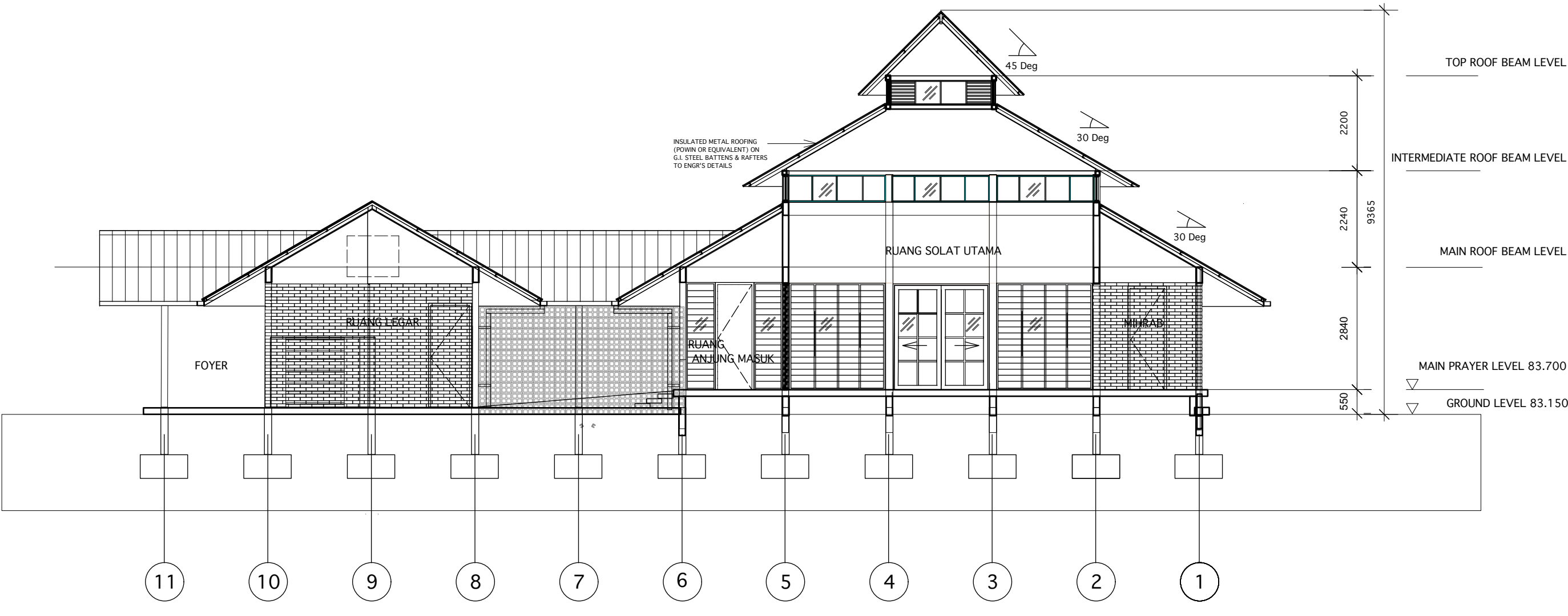
SECTION C-C
