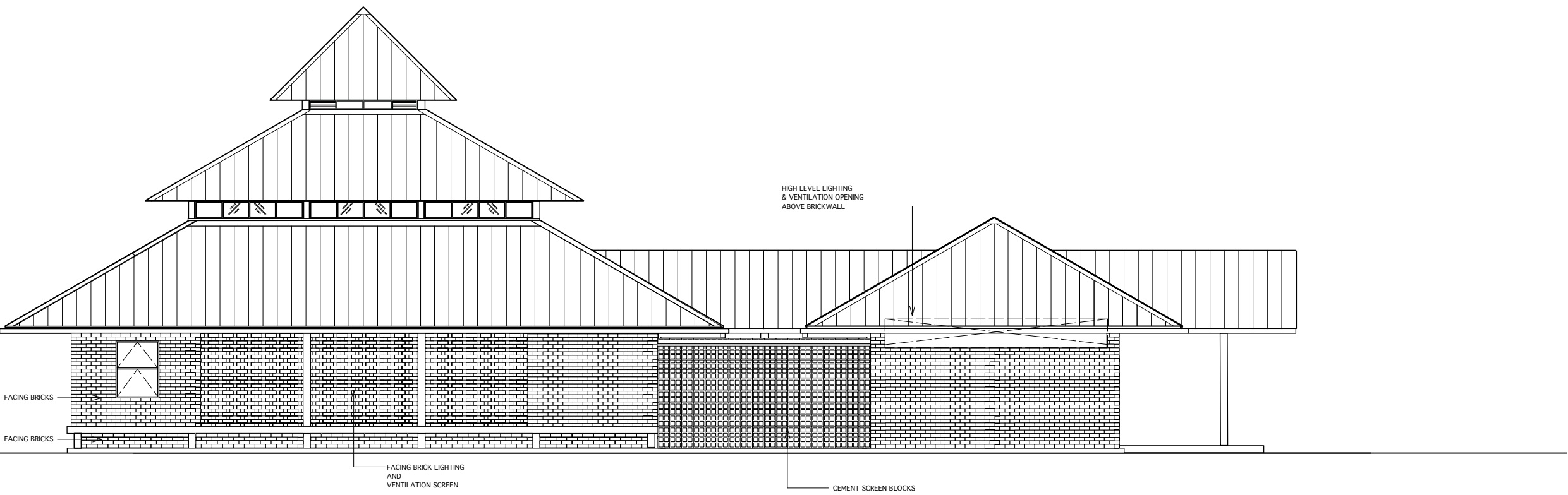
SOUTH ELEVATION
